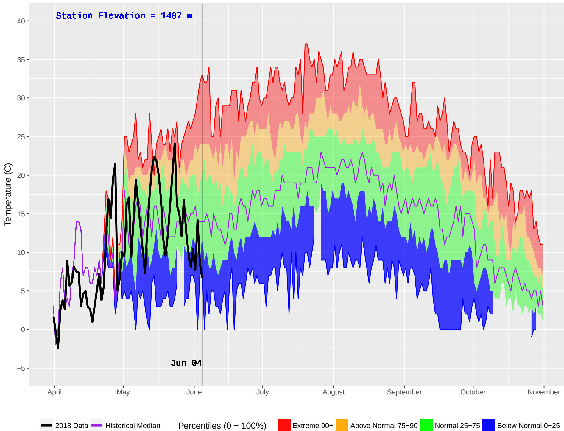
THYNNNE (279) : Historical (1977–2016) and Current (2018) Noon Temperature
